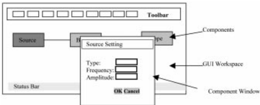
Fig. 6. The layout of the client GUI.
