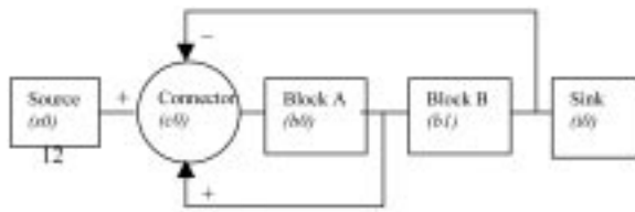
Fig. 3. Control system block diagram example.
