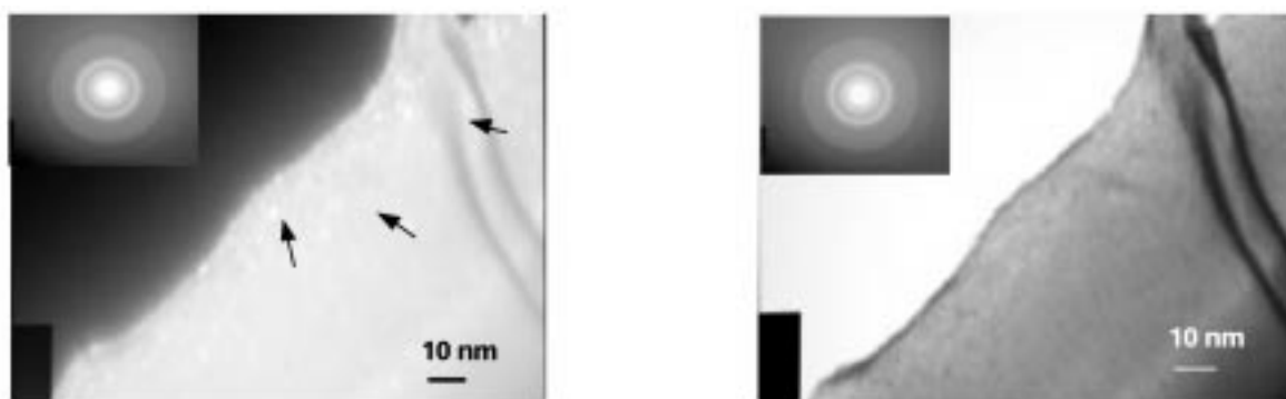
Fig. 2. Physical and optical properties of sol-gel nano-silver doped silica film on glass substrate as a function of heat-treatment temperature. TEM images obtained by REU 2002 student of \text{SiO}_2 gel containing 0.05% Ag, with inset diffraction patterns of Ag particles (see Journal of Applied Physics , 93 (2003), pp. 9553–9561).
