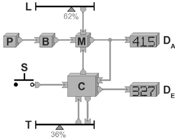
Fig. 1. Example schematic for cruise control (The enclosing graphical user interface of the ShelbySim application is ordinary and uninteresting. For clarity, this figure is extracted from it, and connection labels and other descriptive elements are omitted).
