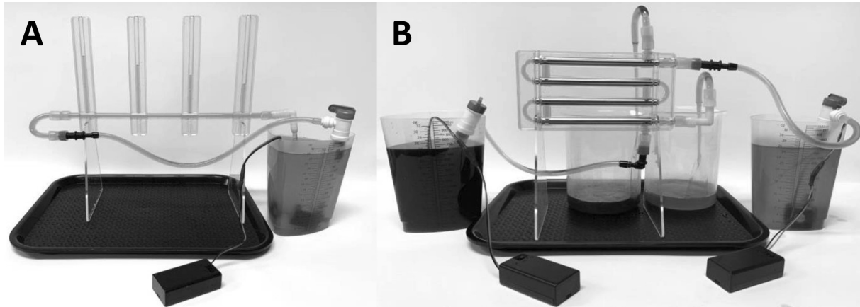
Fig. 1. (A) Hydraulic loss module and (B) double pipe heat exchanger experimental set ups used in hands-on and virtual demonstration implementations.
